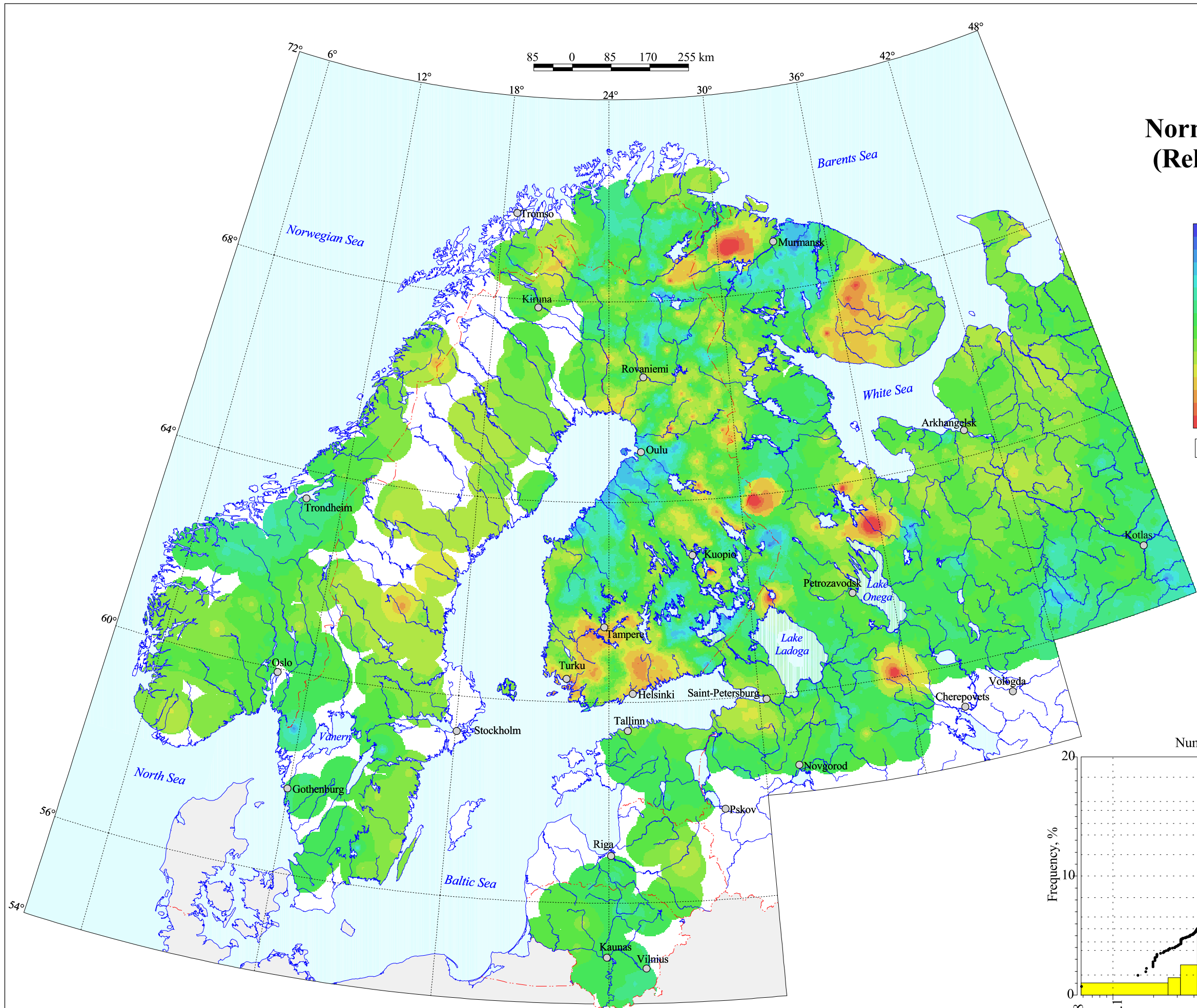
Thallium in Stream Sediment
